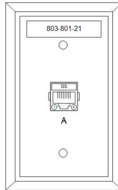
ACCEPTABLE SYMBOLS FOR TYPE E OUTLET
