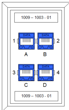
ACCEPTABLE SYMBOLS FOR TYPE D OUTLET
