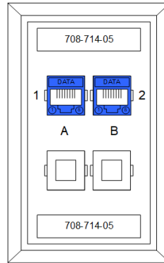
ACCEPTABLE SYMBOLS FOR TYPE B OUTLET
